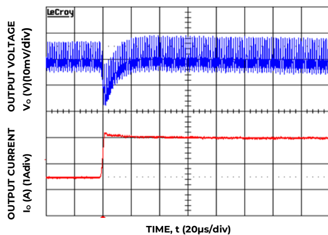
Figure 10. Transient Response to Dynamic Load Change from 50% to 100% at 12V in , C out =1x47μF+1x330μF, C Tune =10nF, R Tune =261
