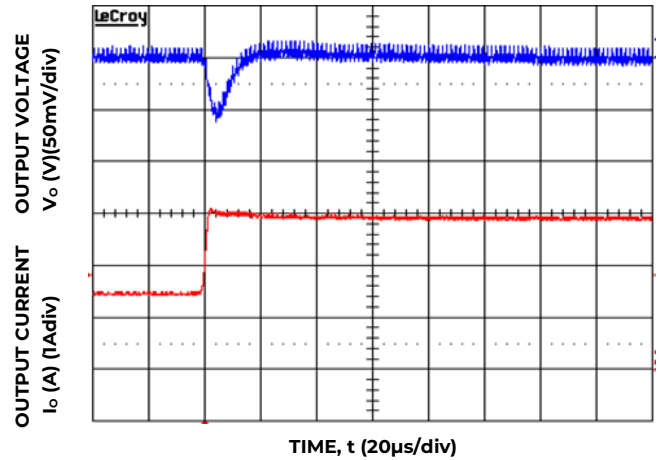
Figure 28. Transient Response to Dynamic Load Change from 50% to 100% at 12V in , C out =2x47μF, C Tune =2200pF, R Tune =261
