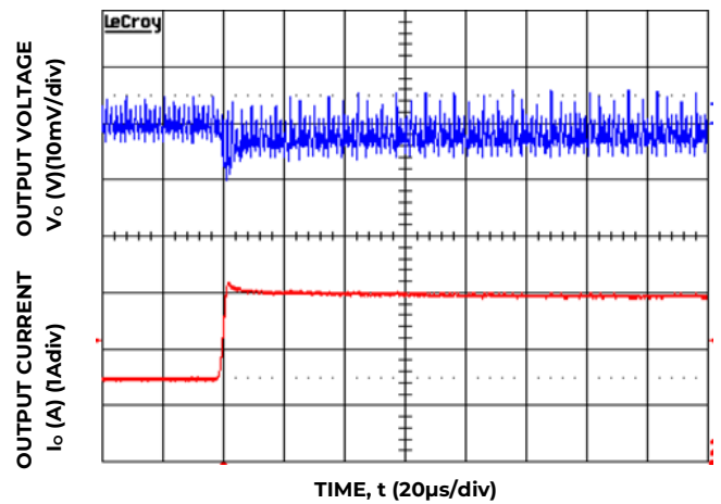
Figure 4. Transient Response to Dynamic Load Change from 50% to 100% at 8V in , C out =1x47μF+2x330μF, C Tune =27nF, R Tune =178
