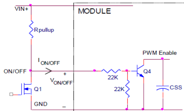
Figure 40. Circuit configuration for using negative On/Off logic
