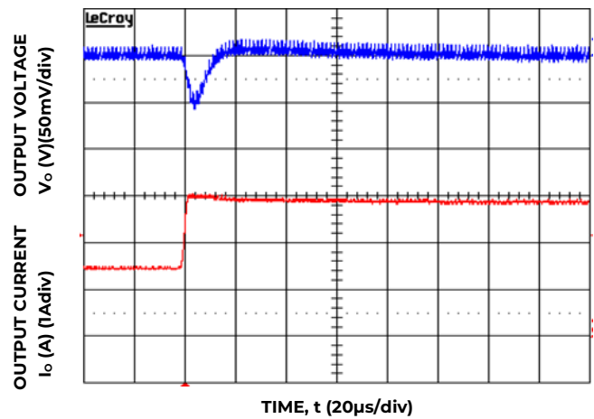
Figure 16. Transient Response to Dynamic Load Change from 50% to 100% at 12V in , C_{out}=2\times 47\mu\text{F} , C_{Tune}=2700\text{pF} , R_{Tune}=261
