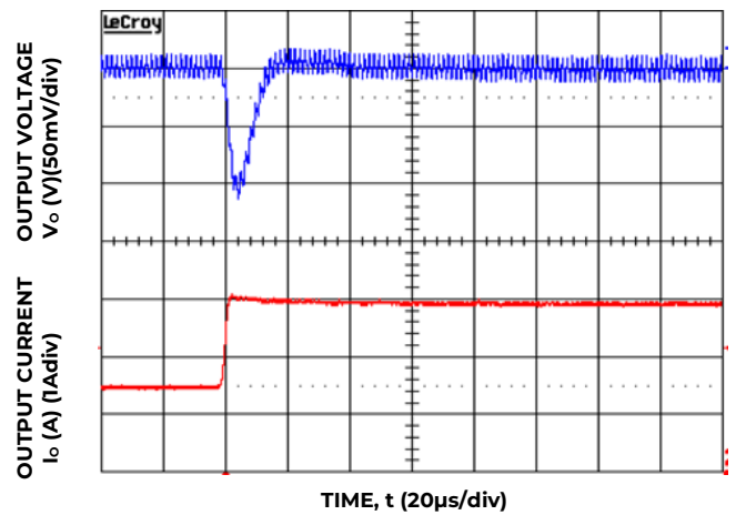
Figure 34. Transient Response to Dynamic Load Change from 50% to 100% at 12V in , C out =1x47μF, C Tune =820pF, R Tune =261
