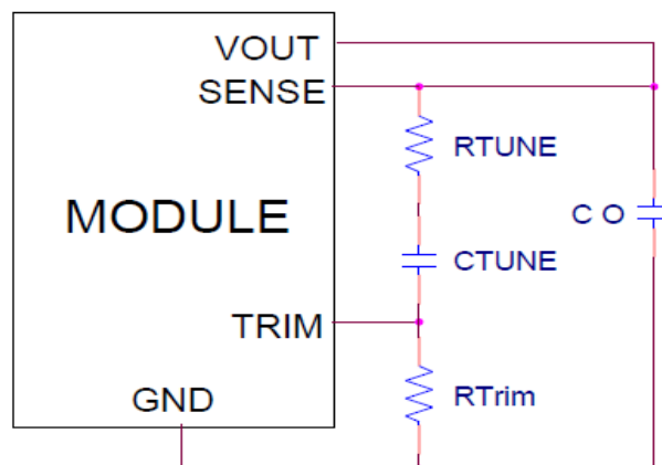
Figure 45. Circuit diagram showing connection of R_{TUNE} and C_{TUNE} to tune the control loop of the module.
