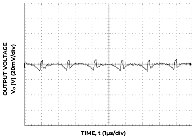
Figure 3. Typical output ripple and noise (C o =10μF ceramic, V IN = 8V, I o = I o,max ).
