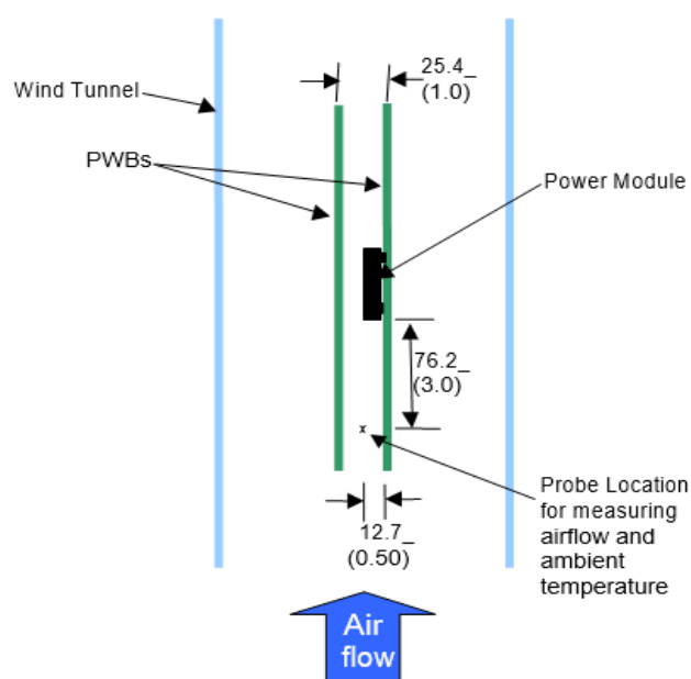
Figure 49. Thermal Test Setup.
