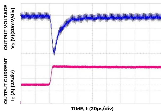
Figure 28. Transient Response to Dynamic Load Change from 50% to 100% at 12V in , C out =3x47μF, C Tune =3300pF, R Tune =178
