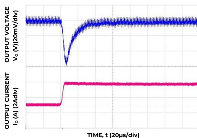
Figure 22. Transient Response to Dynamic Load Change from 50% to 100% at 12V in , C out =3x47μF, C Tune =3300pF, R Tune =178
