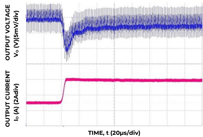
Figure 4. Transient Response to Dynamic Load Change from 50% to 100% at 12V in , C out =1x47μF+4x330μF, C Tune =33nF, R Tune =178
