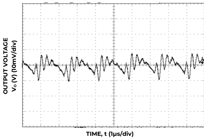
Figure 3. Typical output ripple and noise (C o =22μF ceramic, V IN = 12V, I o = I o,max ).
