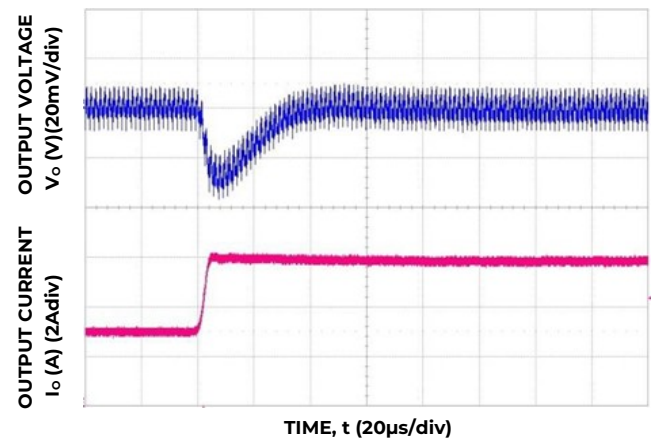
Figure 16. Transient Response to Dynamic Load Change from 50% to 100% at 12V in , C out =1x47μF+1x330μF, C Tune =4700pF, R Tune =178
