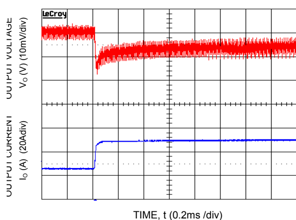
Figure 4. Transient Response to Dynamic Load Change from 50% to 100% at 12V in , C ext = 5x47μF + 22x330μF polymer, C Tune = 330nF, R Tune = 100ohms
