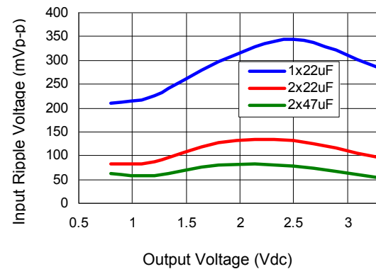
Figure 28. Input ripple voltage for various output voltages with 1 \times 22\mu\text{F} , 2 \times 22\mu\text{F} or 2 \times 47\mu\text{F} ceramic capacitors at the input (30A load). Input voltage is 12V.
