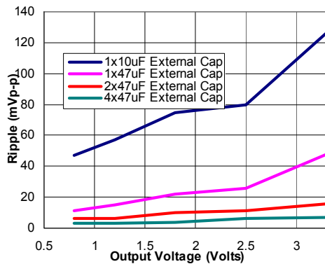
Figure 29. Output ripple voltage for various output voltages with external 1x10 μF, 1x47 μF, 2x47 μF or 4x47 μF ceramic capacitors at the output (30A load). Input voltage is 12V.
