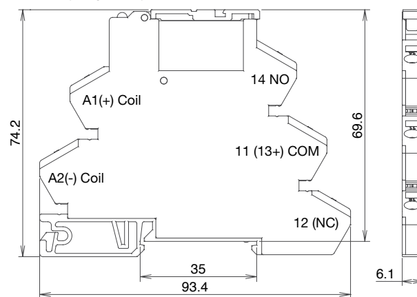
RV8H-S Spring Clamp Terminals
