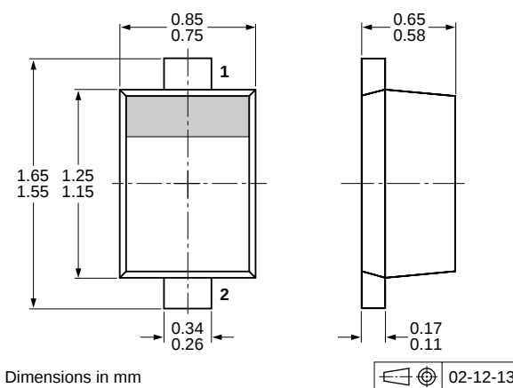
Fig 13. Package outline SOD523 (SC-79)
