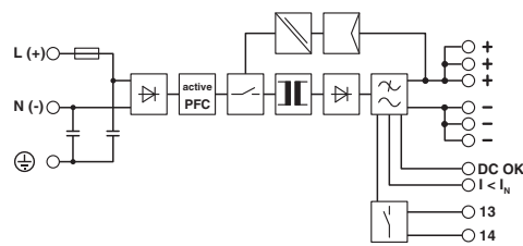
Application drawing
