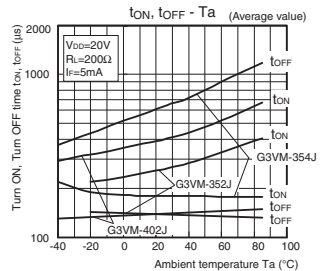
G3VM-352J/354J/402J
