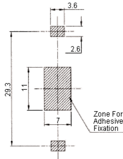
PCB Mounting Layout
