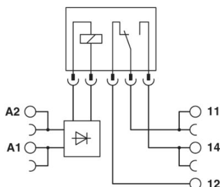
Circuit diagram
