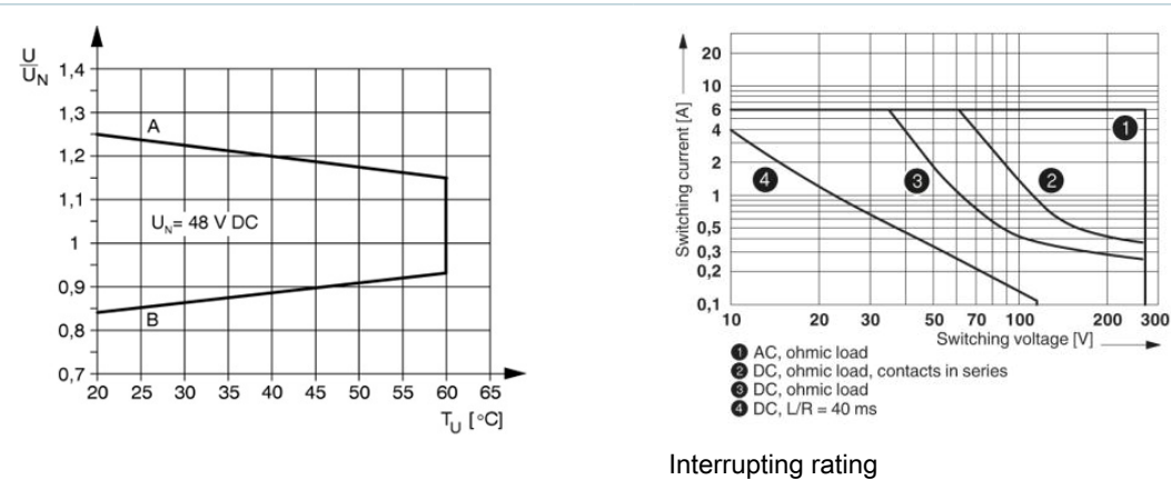
Interrupting rating
