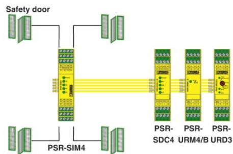
Modular PSR safety relays
