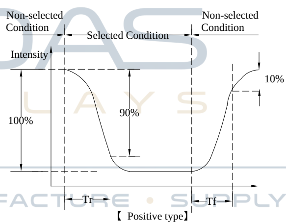
Definition of Response Time (Tr , Tf)
