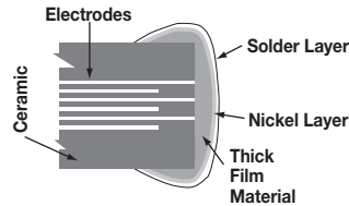
Plated MLV
