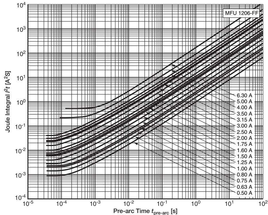
Typical I^2t vs. t_{\text{pre-arc}} characteristic of MFU 1206 (1)
