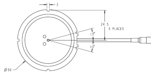
TW2405 Dimensions (mm)
