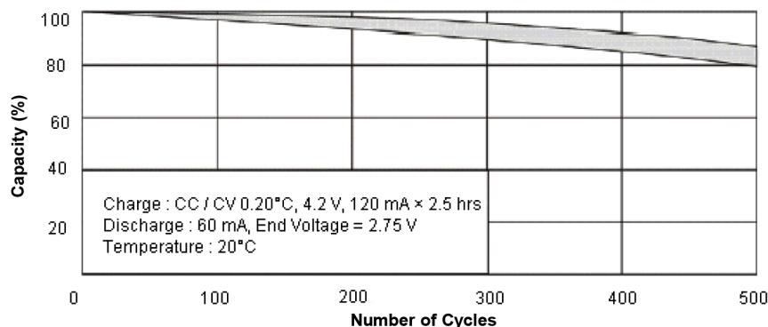
LIR2450 Typical Cycle Life
