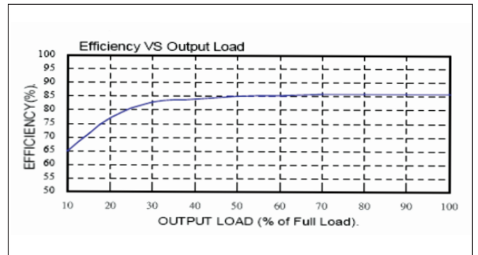
Efficiency / Load Curve DPX30-48WS05
