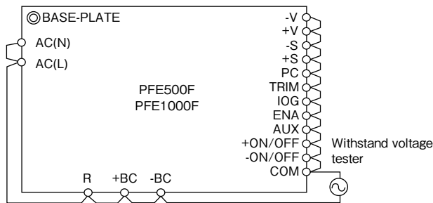
Fig. 21-1 Input to Baseplate Withstand Voltage Test Method
