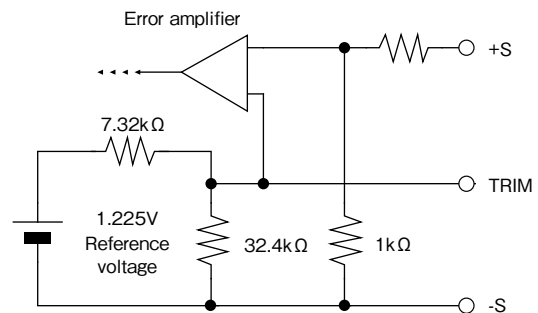
Fig.2-3 Internal TRIM Circuit (For the Reference)
