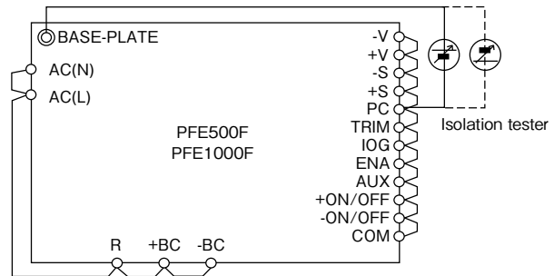
Fig. 22-1 Insulation Resistance Test Method
