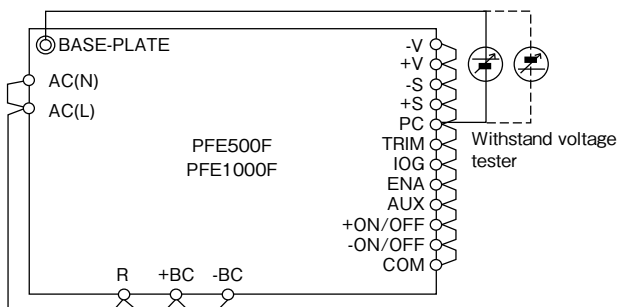
Fig. 21-3 Output to Baseplate Withstand Voltage Test Method
