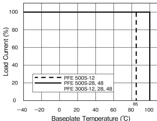
Fig. 12-2 Derating Curve
