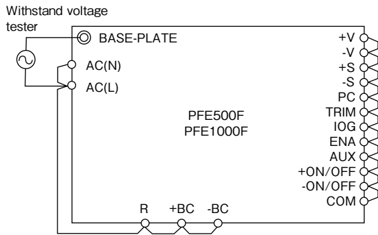
Fig. 21-1 Input to Baseplate Withstand Voltage Test Method
