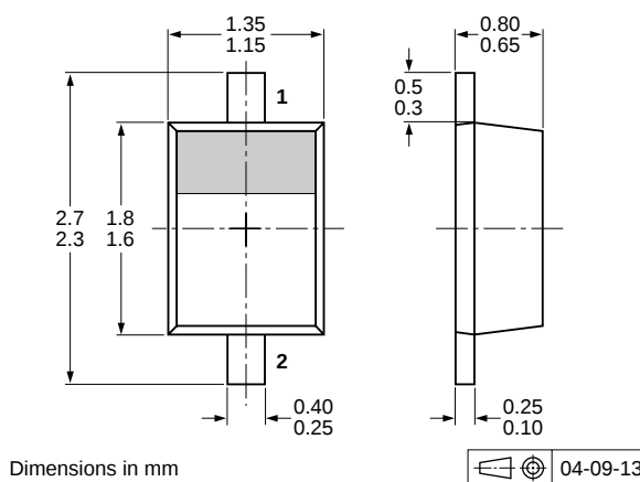
Fig 15. Package outline SOD323F (SC-90)
