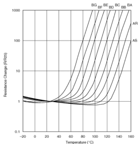
Resistance-Temperature Characteristics
