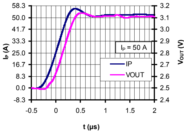
Figure 21: Step response
