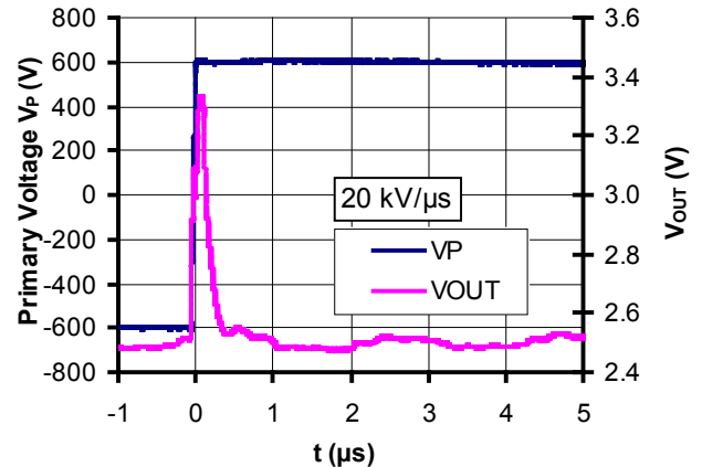
Figure 6: dv/dt
