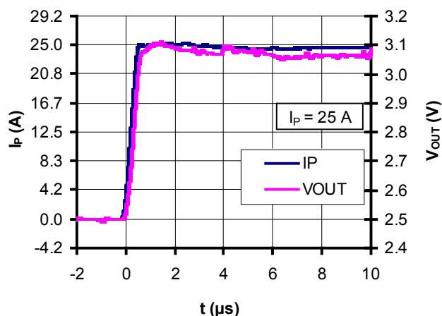
Figure 16: Step response
