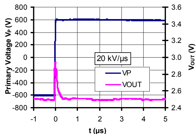
Figure 18: dv/dt
