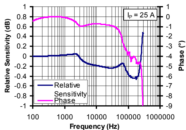
Figure 14: Frequency response
