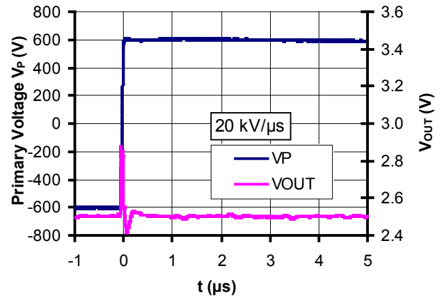
Figure 24: dv/dt
