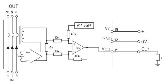
Figure 32: Test connection
