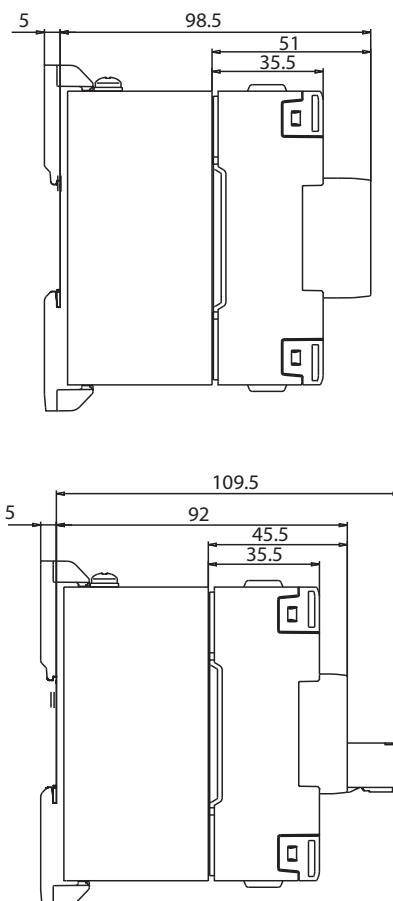
RGS...H51 (RGS on RHS37A heatsink)
