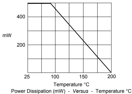
Figure 2 - Derating Curve
