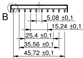
sectional drawing A-A
