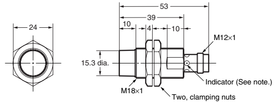
E2A-M18KN16-M1-□□/E2A-S18KN16-M1-□
