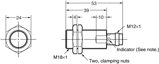
E2A-M18KS08-M1-□□/E2A-S18KS08-M1-□
