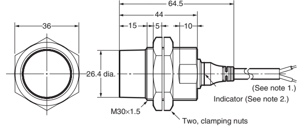
E2A-M30KN20-WP-□□/E2A-S30KN20-WP-□
