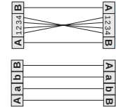
Breakout cable NKO*-BO*
