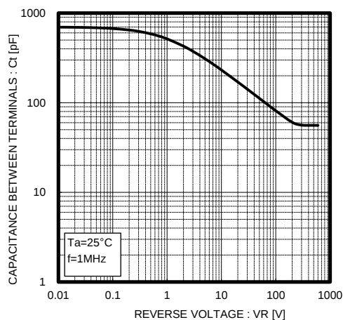
Fig.4 VR-Ct Characteristics
