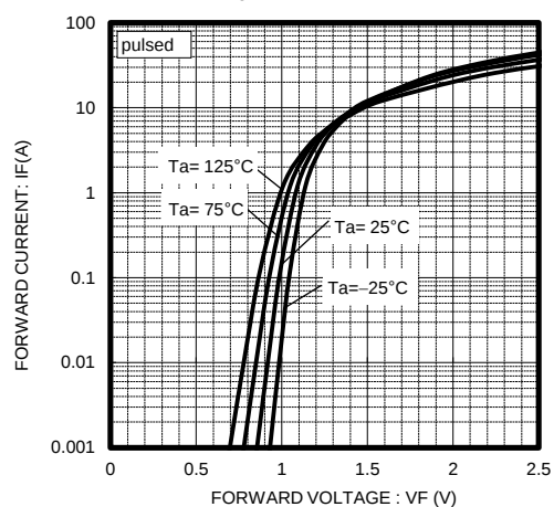
Fig.1 VF-IF Characteristics
