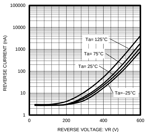
Fig.3 VR-IR Characteristics
