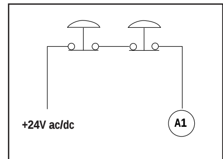
Figure 3. Series connection of multiple E-stop switches
