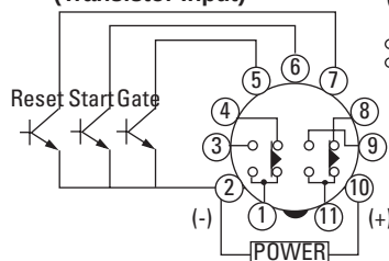
(Transistor Input)
