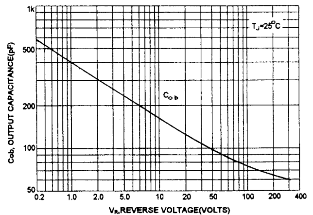
OUTPUT CAPACITANCES
