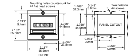
Panel Mount Depth: 2.377"/60.4mm
