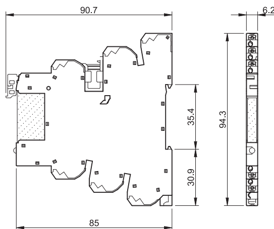
39.90 39.91 Push-in terminal
