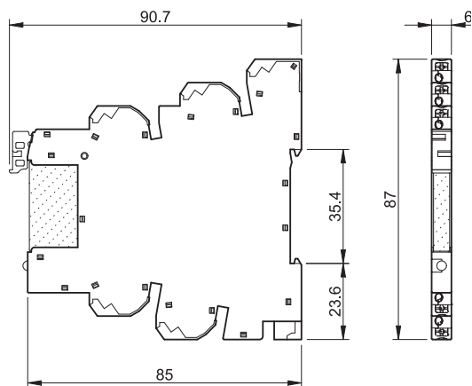
39.70 39.71 Push-in terminal
