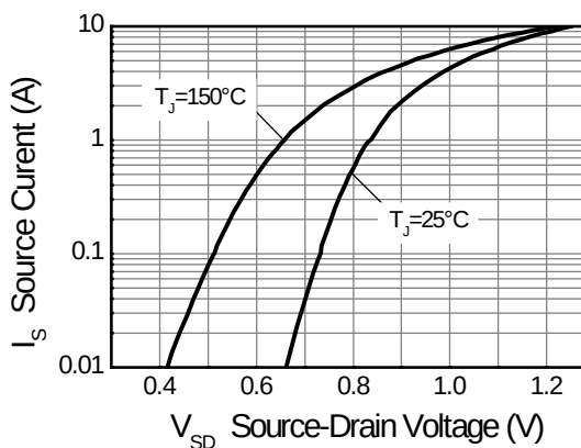
Reverse Diode Characteristic
