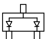
Figure 2, Common Anode
