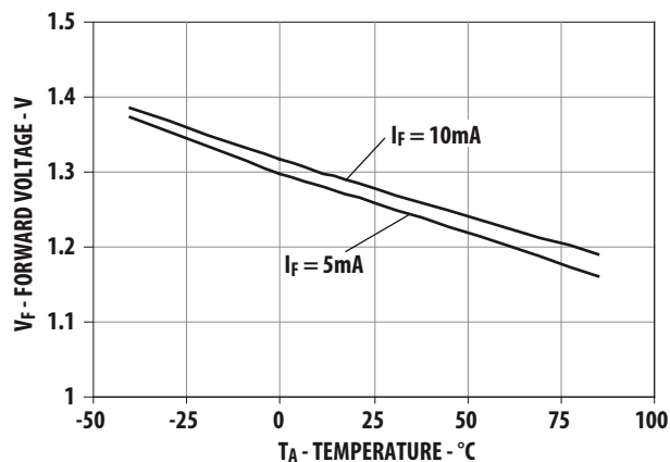
Figure 8. Typical Forward Voltage vs. Temperature
