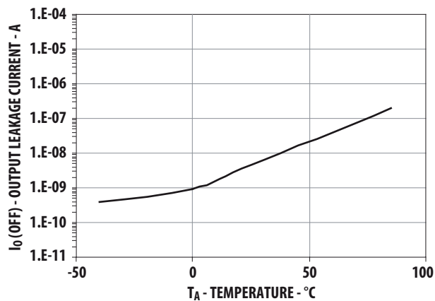
Figure 6. Typical Output Leakage Current vs. Temperature
