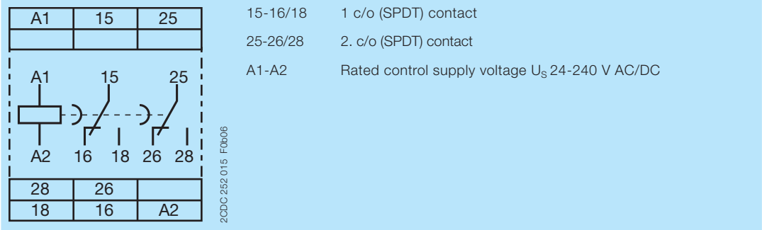
Connection diagram
