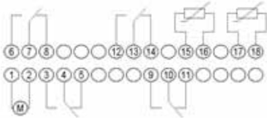
DTS/PRG-SW: simple installation
