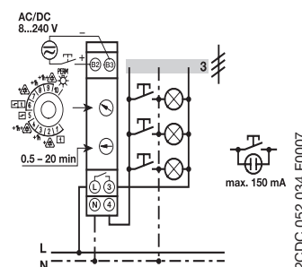
E 232E-8/230 Multi 10 3 conductor
