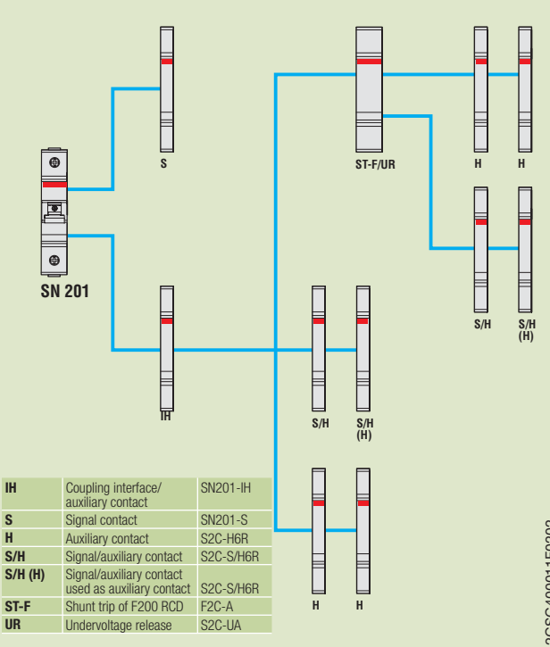
Combination of auxiliary elements with SN 201
