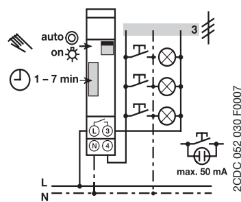
E 232-230 3 conductor
