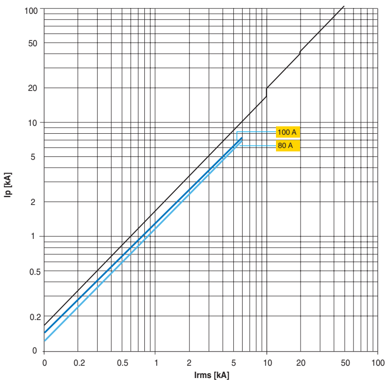
S 280 80-100 A, characteristic C
