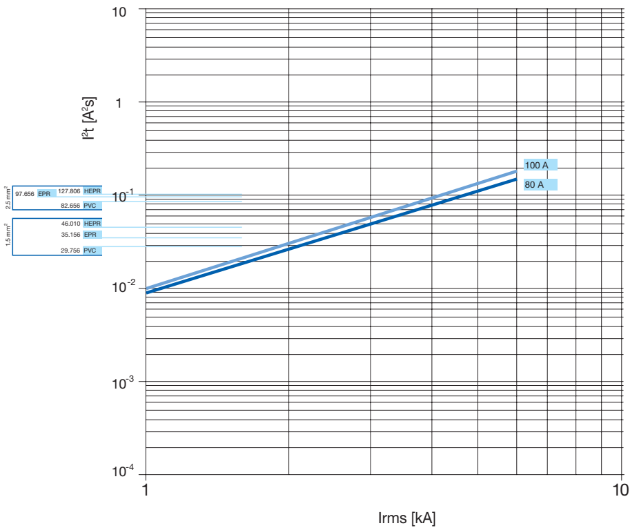
S 280 80-100 A, characteristic B 230/400 V let-through energy
