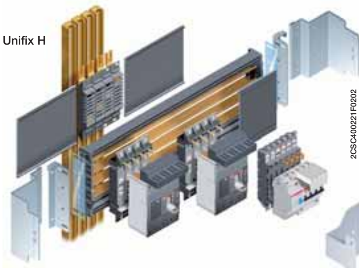
Unifix L
