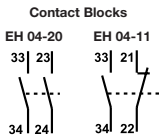
EH 04-20
