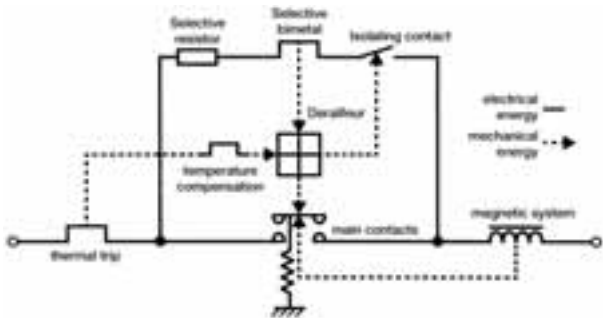
Functional diagram of selective main circuit breakers S 700
