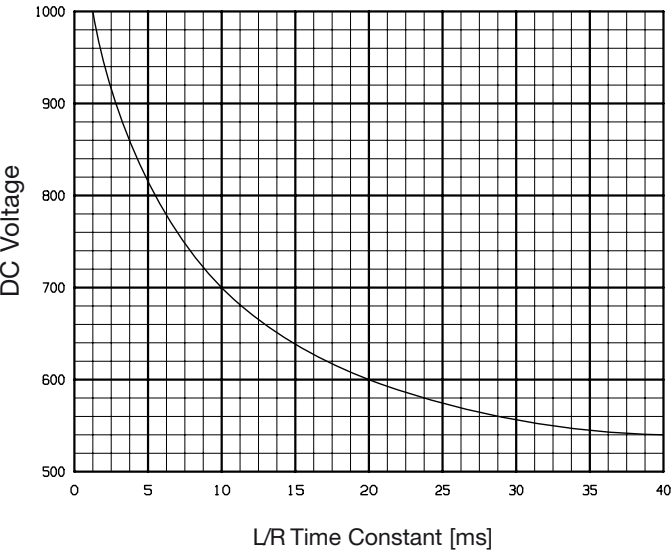
Voltage capabilities vs. time constant
