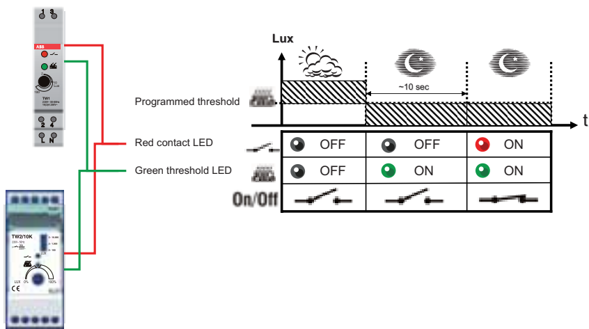
TW1 and TW2/10K operating principle
