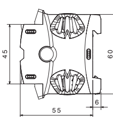
ISS 16/3 ISS 63/3
