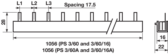
PS 3/60
