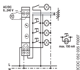
E 232E-8/230 Multi 10 4 conductor
