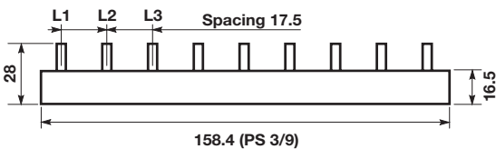
PS 3/9
