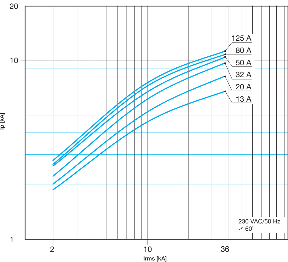
S 800 N characteristics B, C and D
