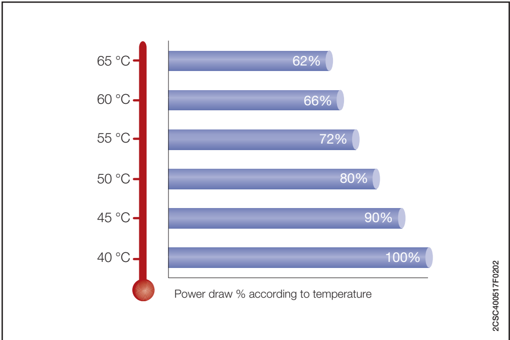
Power draw according to temperature and altitude
