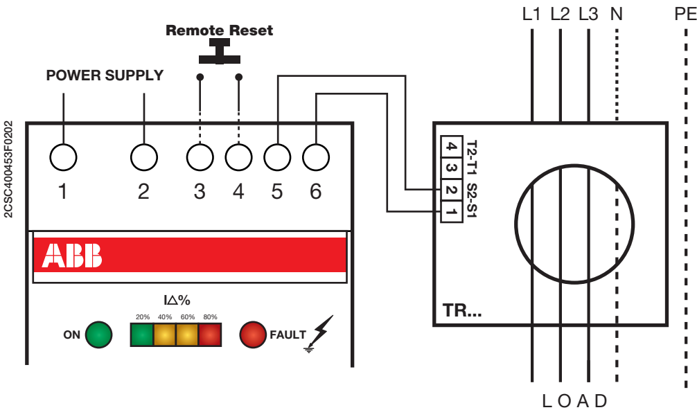
Toroid - relay connection
