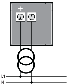
Insertion via VT
