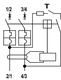
DS202C
