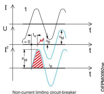
Oscillogram of short-circuit breaks on two circuit-breakers:
