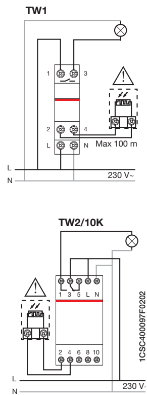
Connection diagram
