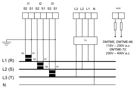
Three-phase with neutral and 3 CTs and 3 VTs Up to 500 V phase-neutral a direct connection is possible
