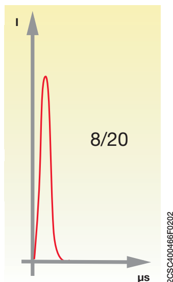
Type 2 Surge Arresters I_{max} : current wave
