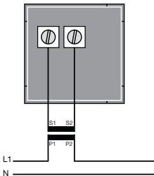
Insertion via CT
