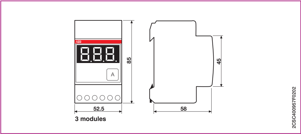
Digital measurement instruments VLMD-1-2, AMTD-1, AMTD-2, VLMD-1-2-R, AMTD-1-R, AMTD-2-R
