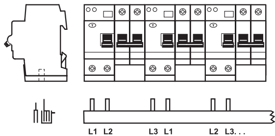
PS 3/26/16H-DDA 202 DS 202 + S2C-S/H6R + DS 202 + S2C-S/H6R + DDA 202 + S 202 + S2C-S/H6R + DDA 202 + S 202 + S2C-S/H6R ...
