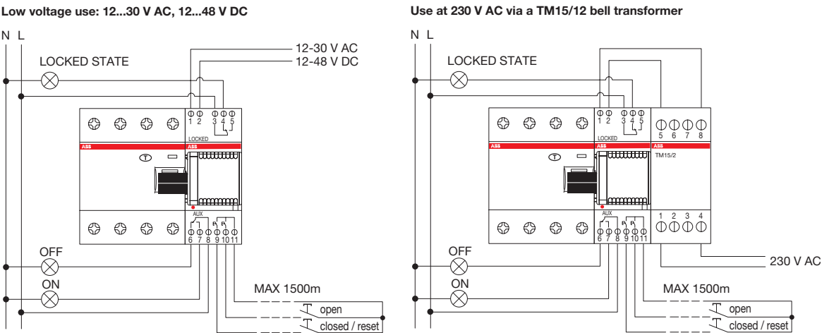
Wiring diagrams for motor operating device F2C-CM and F2C-ARI auto-reclosing unit
