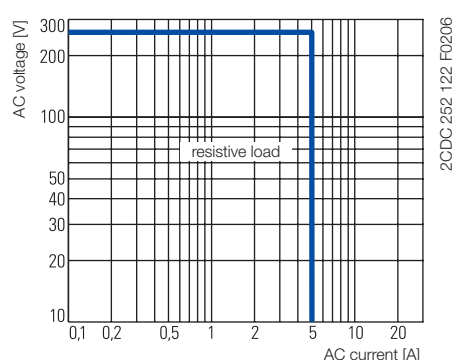
CT-D.2x
