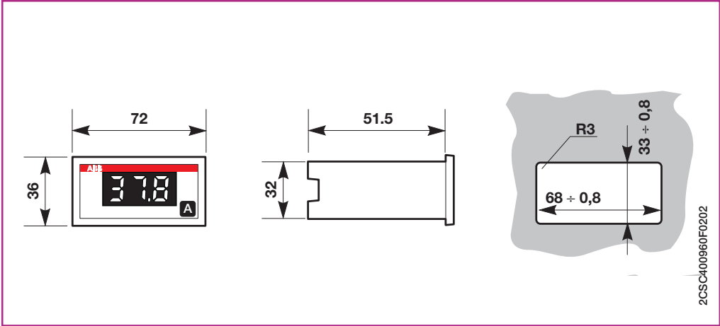
Front panel analogue measurement instruments VLMD P, VLMD-R P, AMTD-1 P, AMTD-1-R P, AMTD-2 P, AMTD-2-R P
