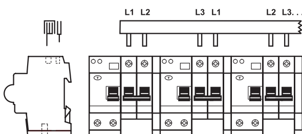
PS 3/28/16 H-DDA 202 T DS 202 + S2C-S/H6R + (DDA 202 + S 202) + S2C-S/H6R ...
