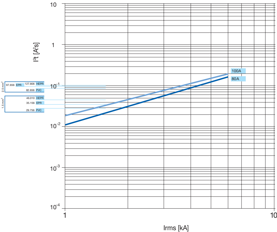
S 280 80-100 A, characteristic C 230/400 V let-through energy
