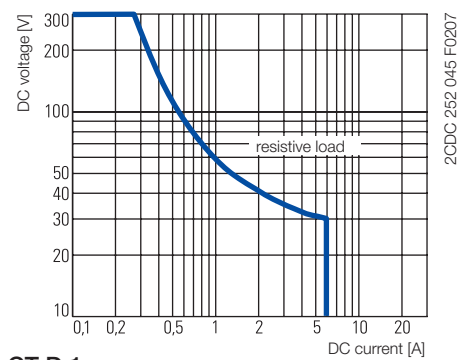
CT-D.1x
