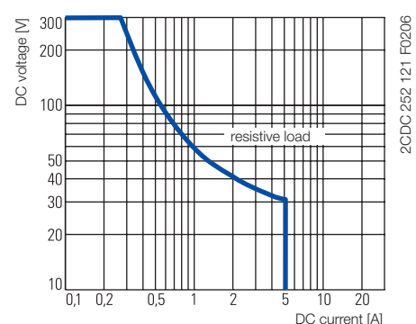
CT-D.2x
