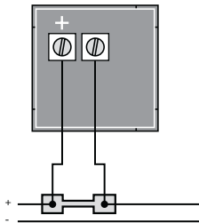
Insertion with Shunt
