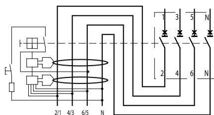
DDA 204 B type
