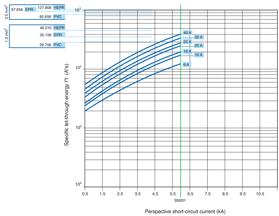
SN201, characteristics D 230 V let-through energy
