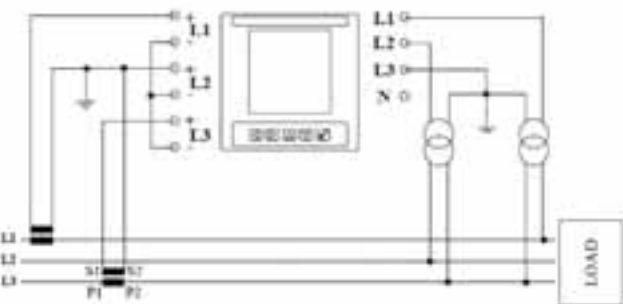
Insertion with 2 CTs and 2 VTs (Aron)
