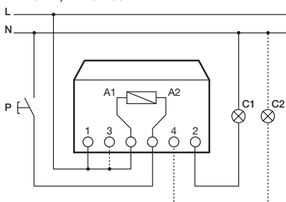
FLR5-12, FLR5-230
