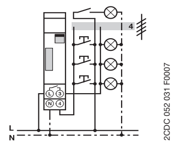
E 232-230 4 conductor
