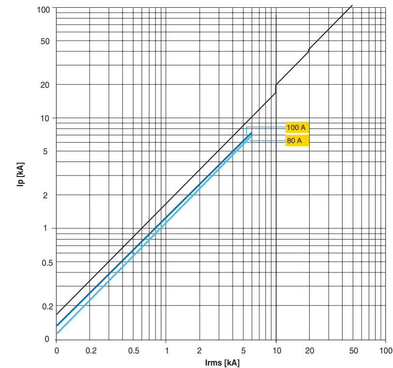
S 280 80-100 A, characteristic B
