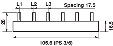
PS 3/6
