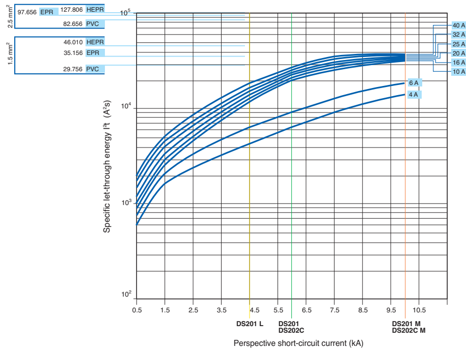
DS201 L - DS201 - DS201 M DS202C - DS202C M, characteristics B and C 230 V let-through energy
