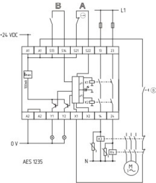
Wiring example
