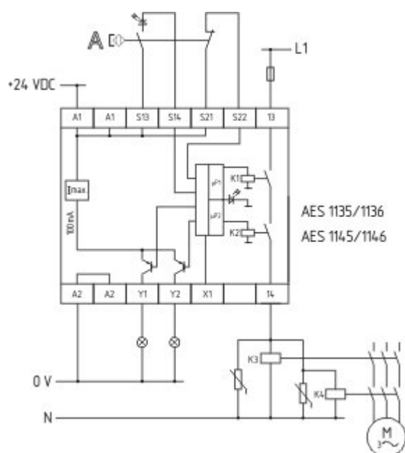
Wiring example
