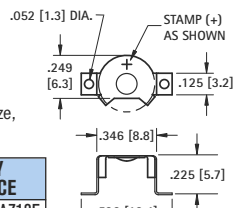
Mounting Detail
