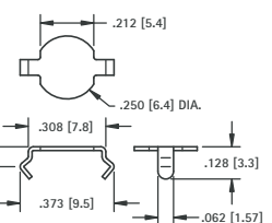
Mounting Detail
