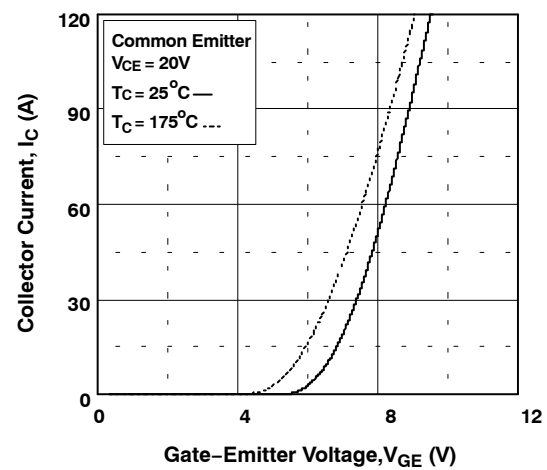
Figure 4. Transfer Characteristics
