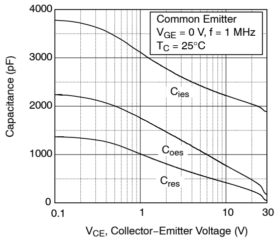
Figure 9. Capacitance Characteristics
