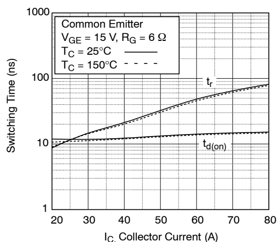
Figure 14. Turn-On Characteristics vs. Collector Current
