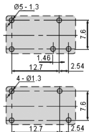
Mounting Hole Layout
