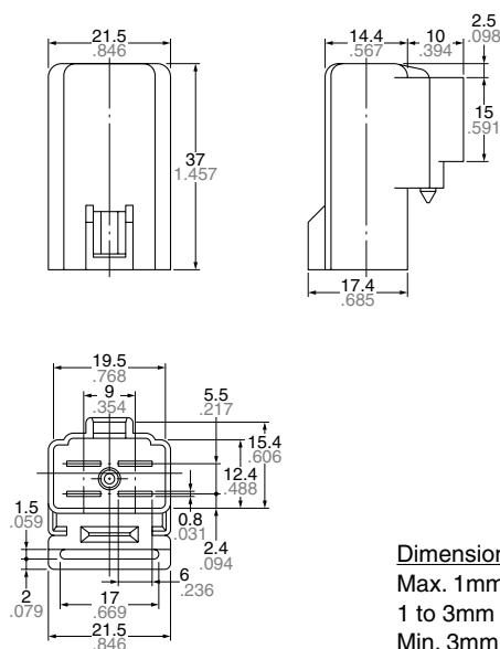
External dimensions
