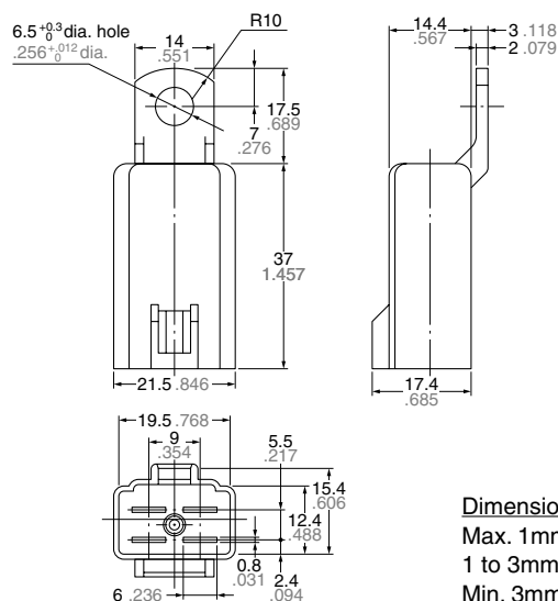
External dimensions
