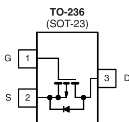
Top View Si2333DS (E3)* * Marking Code
