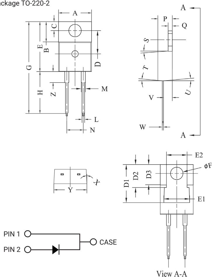
Package TO-220-2
