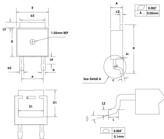
Package TO-252-2
